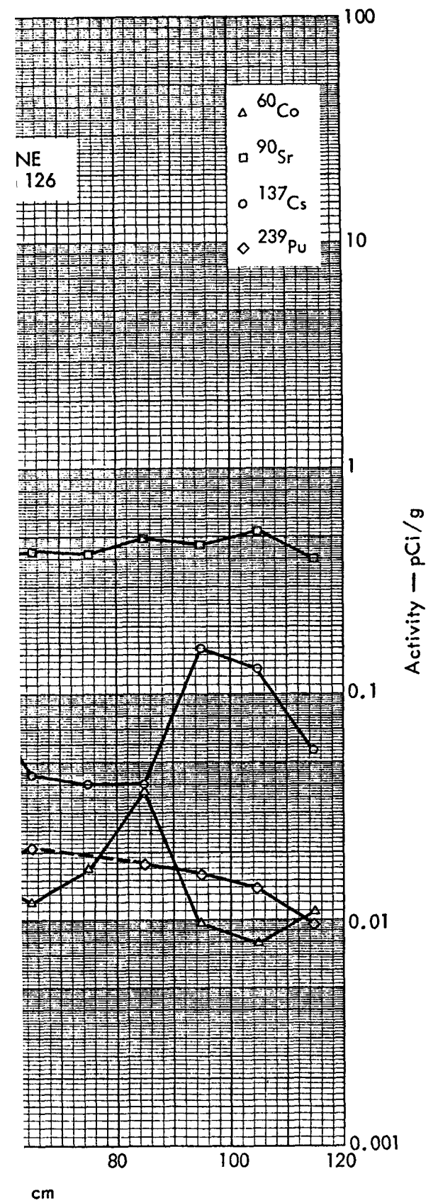
ACTIVITIES OF SELECTED RADIONUCLIDES AS A FUNCTION OF SOIL DEPTH
